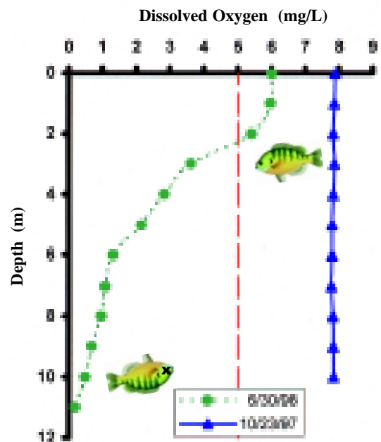
WEISS LAKE OXYGEN PROFILE AT DAM Fall of 1997 and Summer of 1998
